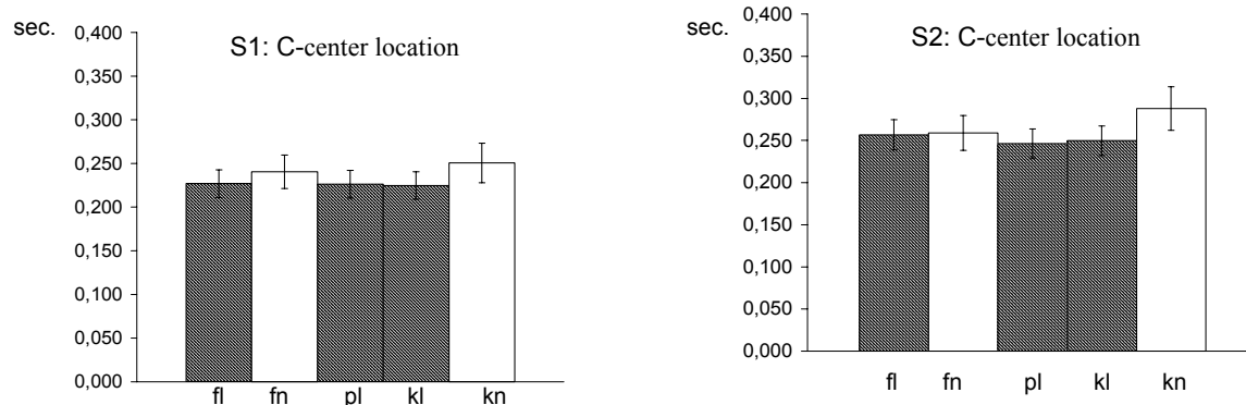
Fig. 3. Mean location of the C-center relative to the burst of the final stop; error bars show the standard deviation (time in sec.).
