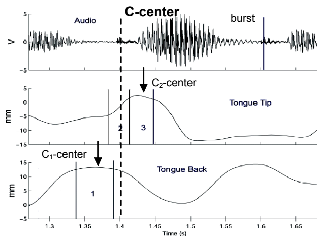
Fig. 1. Kinematic parameter extraction (illustration only) in one production of claque . Top: audio; middle: vertical TT-movement; bottom: vertical TB-movement. 1 = C 1 constriction plateau; 2 = C 2 closing gesture; 3 = C 2 constriction plateau; C-center aligned relative to the acoustic burst of the word-final consonant (see text for details).
