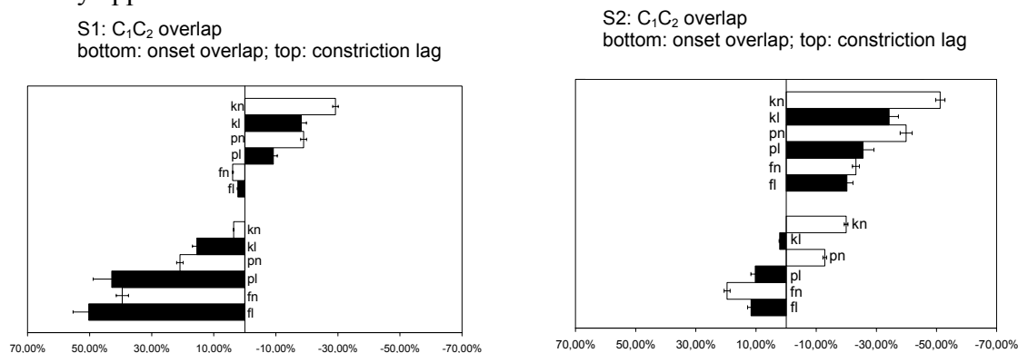
Fig. 2. Mean values and standard deviation (in %) of C 1 C 2 overlap indices. Positive values indicate more overlap, negative values indicate greater lag between C 1 and C 2 (see text for details).
