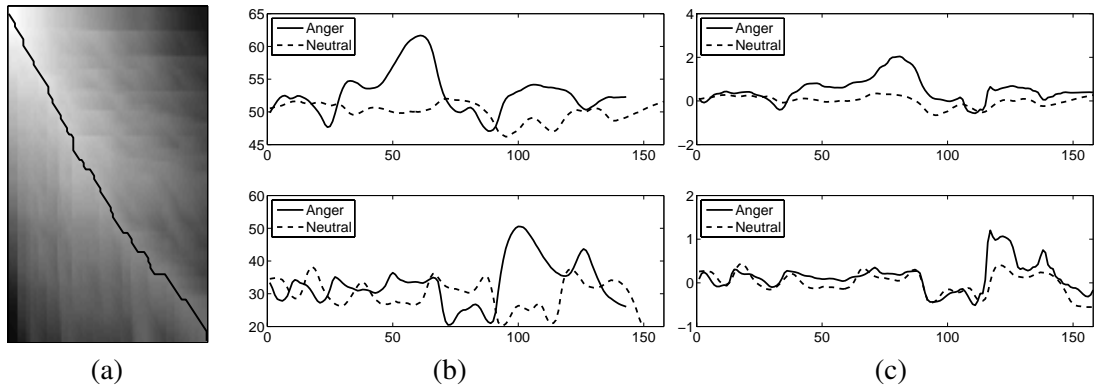
Figure 3: Dynamic time warping to align neutral and emotional facial features. (a) optimum alignment path (b) original lip features (c) normalized and warped lip features.
