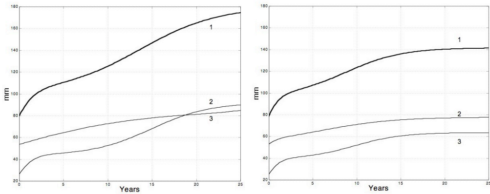
Figures 7. Vocal tract length (1), pharyngeal cavity length (2), and oral (mouth) cavity length (3) for male (left panel) and female (right panel). It is noticeable that for male speakers, the pharyngeal cavity length reaches and even exceeds that of the oral cavity, which is not the case for female speakers.
