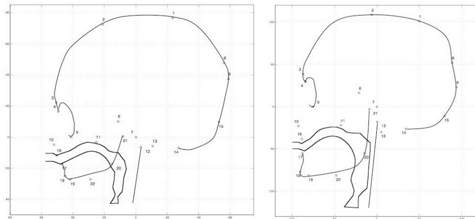
Figure 6. Modeling of the growing vocal tract positioned relative to Fenart's anthropometric landmarks (left panel: newborn, right panel: adult male). Anthropometric landmarks are those reported in Figure 2. The straight line from the basion (point 12) roughly represents the position of the anterior part of the cervical vertebrae and its inclination relative to the skull. Note that the pharyngeal wall gets closer to the vertebrae during childhood.
