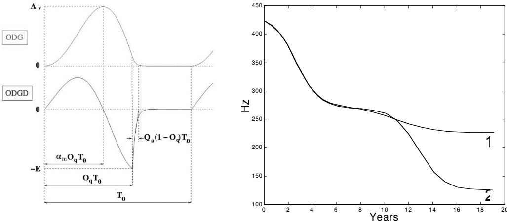
Figure 5. Left: Generic model of the glottal source and control parameters. T_0 , fundamental period; A_v , voicing amplitude; O_q , open quotient ; \alpha_m , asymmetry coefficient; Q_a , return phase quotient; E , amplitude of the maximum excitation (following Henrich, 2001). Right: Prototypical F_0 variations for male and female speakers from birth to adulthood. Double logistic curves have been fitted to those variations.
