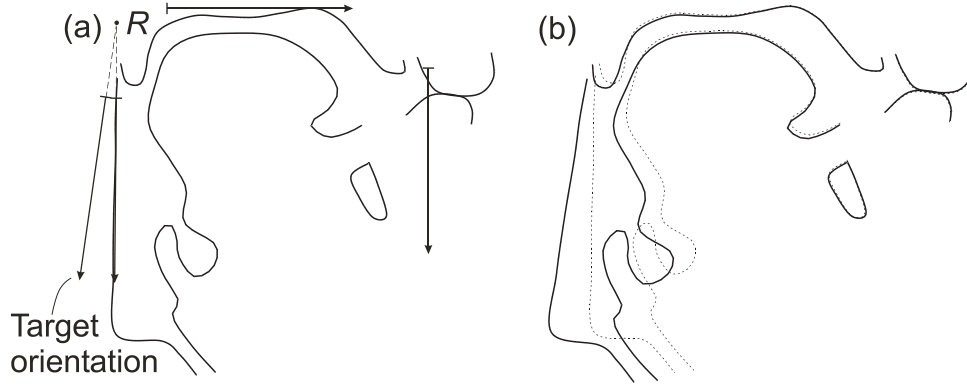
Figure 2. Warping of the MRI-tracing of the consonant /b/ in /ubu/.
